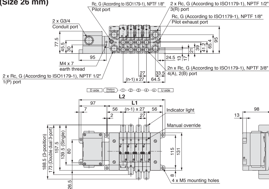
Dimension [mm]
