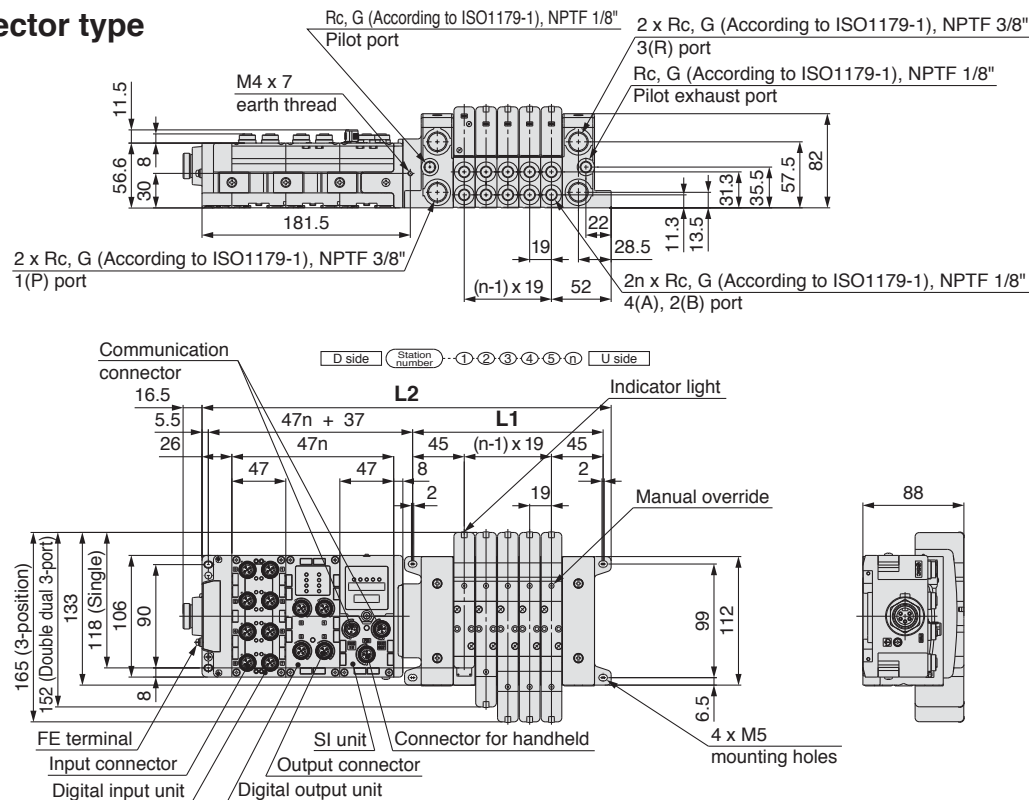
Formula: L1 = 19n + 71 , L2^{Note) = 19n + 167.5} n: Stations (Maximum 16 stations)
