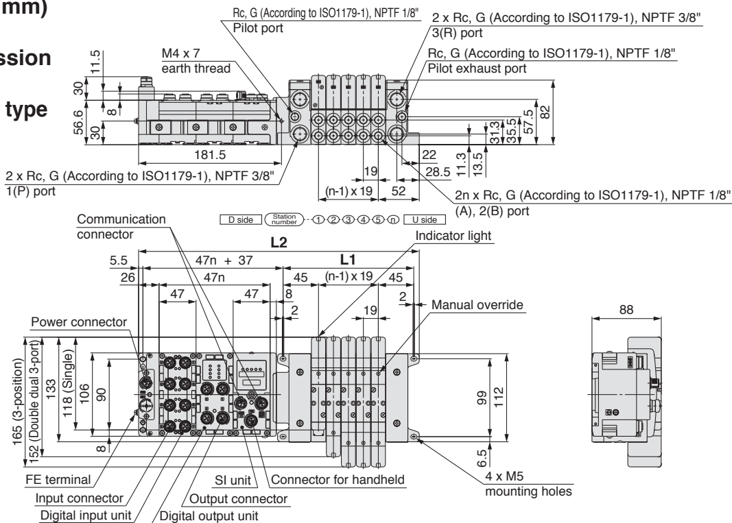
Formula: L1 = 19n + 71 , L2^{Note) = 19n + 167.5} n: Stations (Maximum 16 stations)
